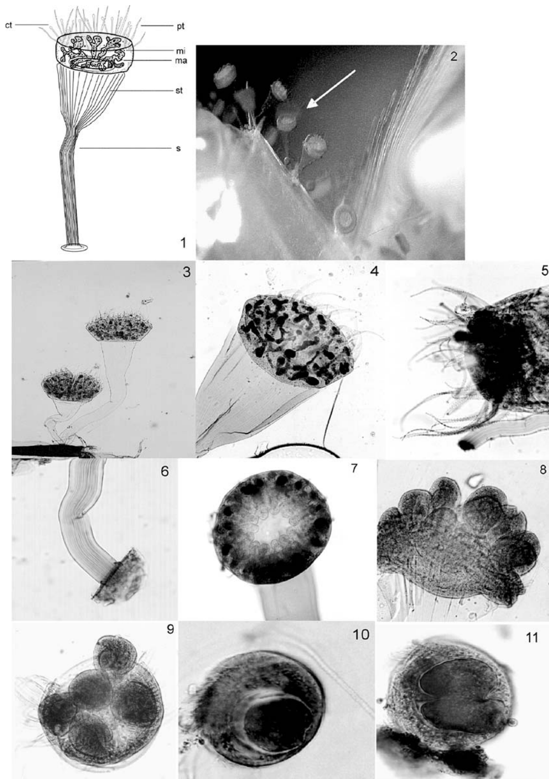
FIGURE 1. Ephelota plana . 1: scheme, ct: capitate tentacles, ma: macronucleus, mi: micronucleus, pt: prehensile tentacles, s: stalk, st: striations; 2: “in vivo” on a pereopod of Gammarus wilkitzkii (arrow) ( \times 35 ); 3: habitus ( \times 100 ); 4: anterior end of the body showing suprastylar zone of stalk and macronucleus ( \times 200 ); 5: apical end of the body with tentacles ( \times 220 ); 6: posterior end of the stalk with striations and basal disk ( \times 250 ); 7: early phase of reproductive stage with numerous buds in the center ( \times 220 ); 8: lateral view of buds showing their ciliar fields ( \times 280 ); 9: apical end of the body with five emerging buds ( \times 230 ); 10: early stage of the swarmer with one single macronucleus ( \times 750 ); 11: advanced phase of the swarmer with the macronucleus under division ( \times 750 ); 12: early developmental stage of adult after settling on the basibiont, with only short capitate tentacles ( \times 180 ); 13: subsequent developmental stage of adult with the macronucleus well differentiated; 14: scheme of “resistant” stage, abbreviations see 1; 15: habitus of “resistant” stage ( \times 100 ); 16: apical end of “resistant” stage with folded tentacles ( \times 250 ); 17: apical end of “resistant” stage showing the shape of the macronucleus ( \times 250 ). Figure continued on next page.
