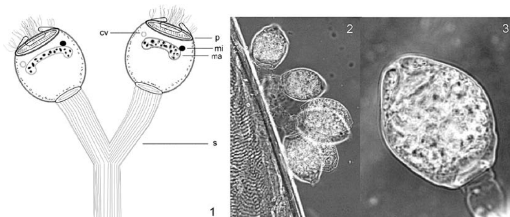
FIGURE 5. Epistylis sp. 1: scheme, cv: contractile vacuole, ma: macronucleus, mi: micronucleus, p: peristomial disk, s: stalk; 2: habitus of a colony on the surface of Gammarus wilkitzkii (×320); 3: zooid showing stalk and peristomial lip (×830).
